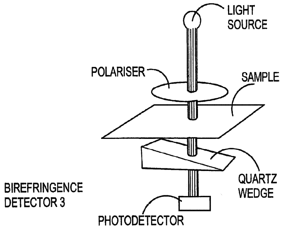
FIG. 3 (PRIOR ART)
