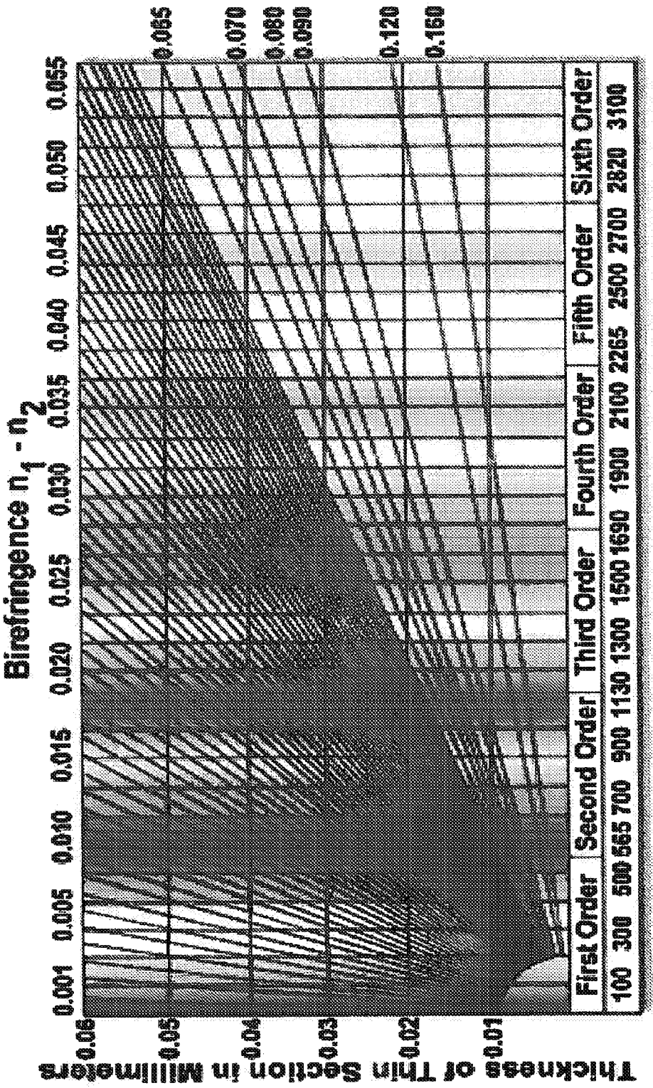
Michel-Levy chart
