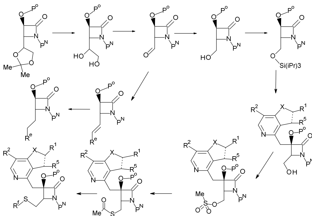
[Chemical Formula 10]
