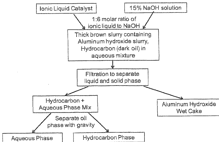
Figure 1 Hydrolysis of Ionic Liquid Catalyst
