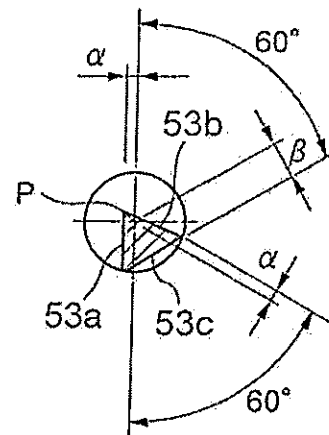
C-C cross section
