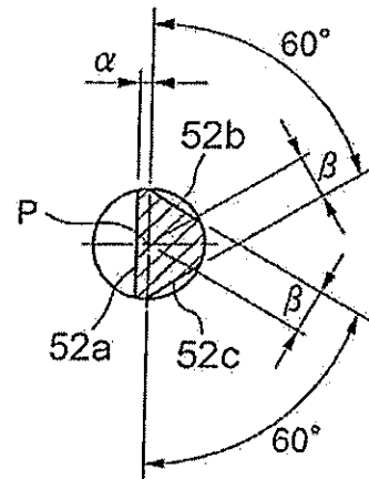
B-B cross section
