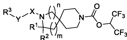
Formula (III);
