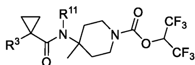
Formula (IIc);
