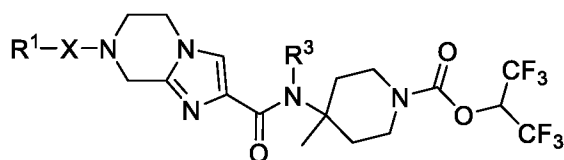
Formula (IV);
