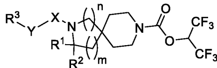
Formula (III);
