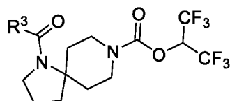
Formula (Id);
