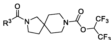
Formula (Ib);
