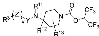
Formula (II);
