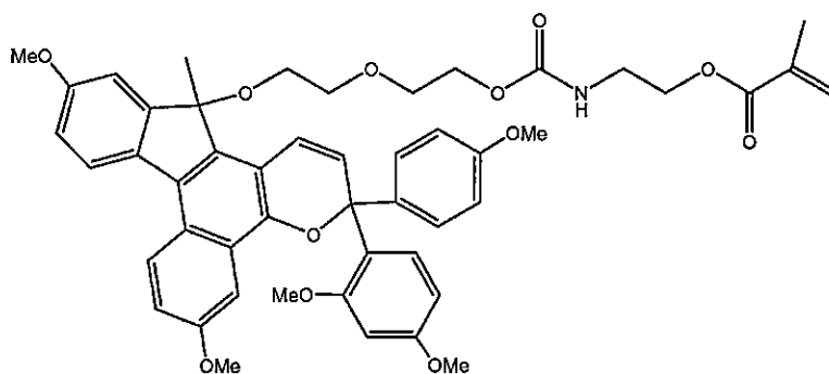
Photochromic compound I
