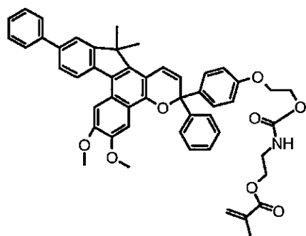
Photochromic compound XII
