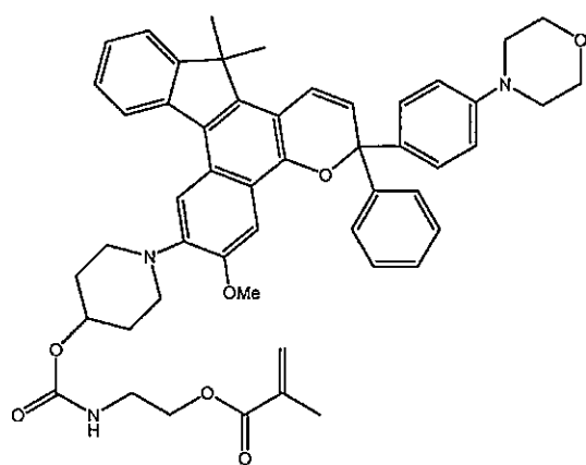
Photochromic compound XI
