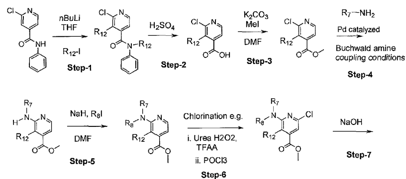
Scheme 8'
