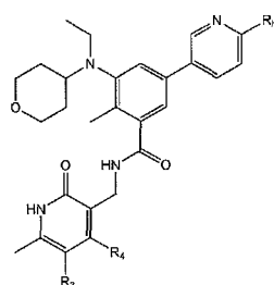
(IIIe),
