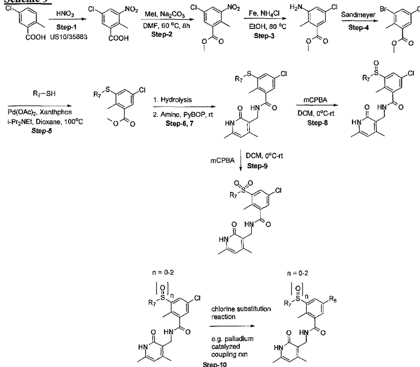
Scheme 9'
