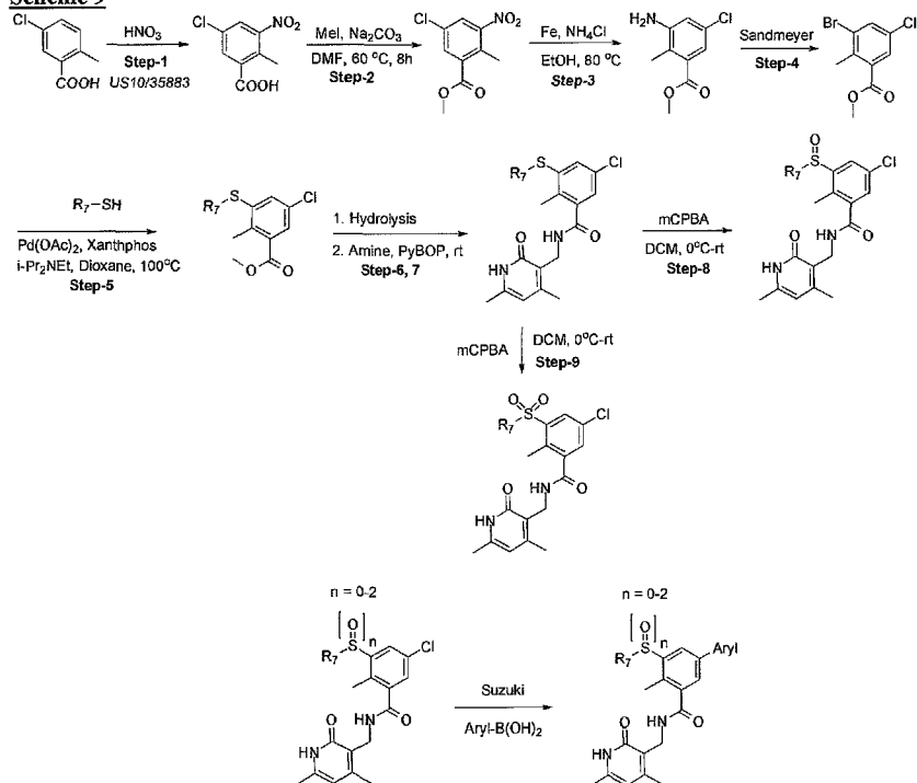
Scheme 9
