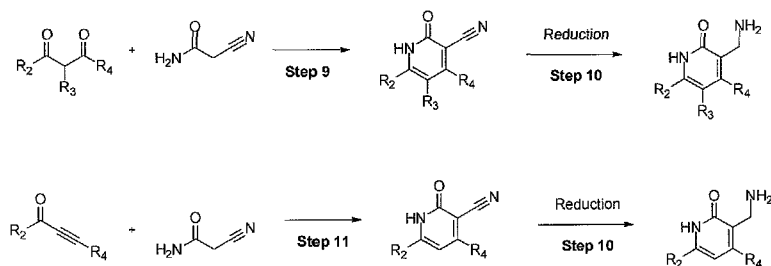
Scheme 6
