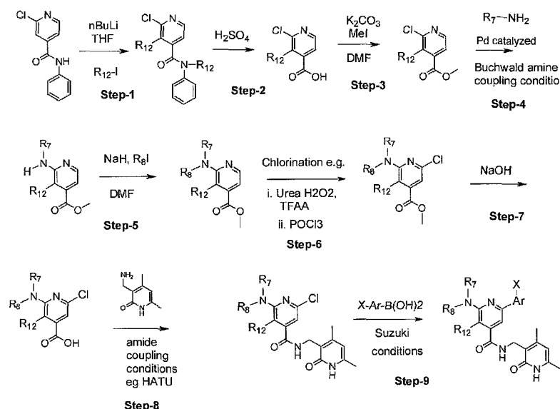
Scheme 8
