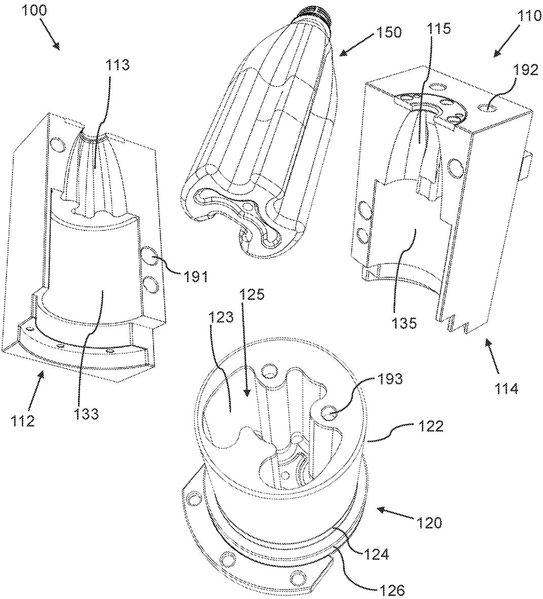
FIG. 1A System for Molding
