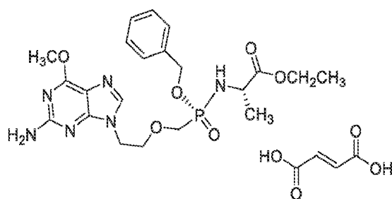
Compound II
