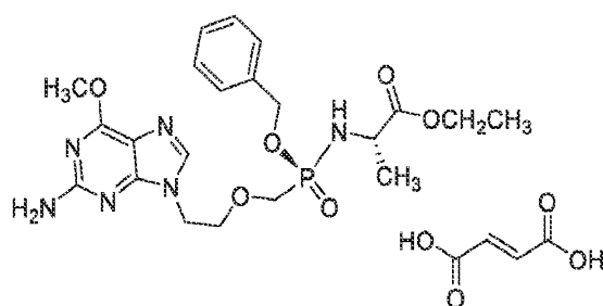
Compound III
