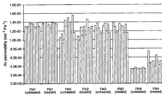
Figure 1 - Air permeability measurements of treated and untreated filtration media
