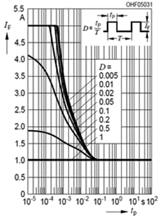
Permissible Pulse Handling Capability I_F = f(t_p) , T_S = 85\text{ }^{\circ}\text{C} , Duty cycle D = \text{parameter}
