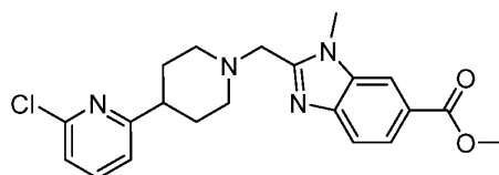
Intermediate 36
