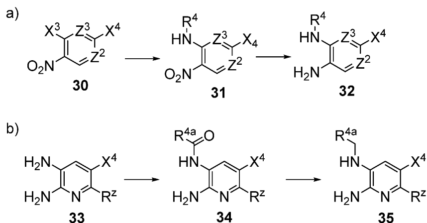
Scheme 8
