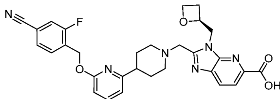
Example 6A-01
