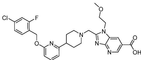
2-((4-(6-((4-Chloro-2-fluorobenzyl)oxy)pyridin-2-yl)piperidin-1-yl)methyl)-1-(2-methoxyethyl)-1H-imidazo[4,5-b]pyridine-6-carboxylic acid hydrochloride
