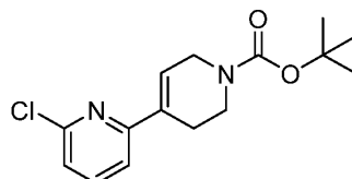
Intermediate 1
