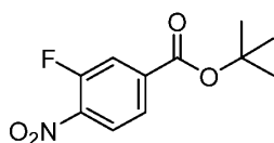
Intermediate 29
