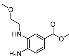
Intermediate 18
