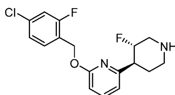
Intermediate 10
