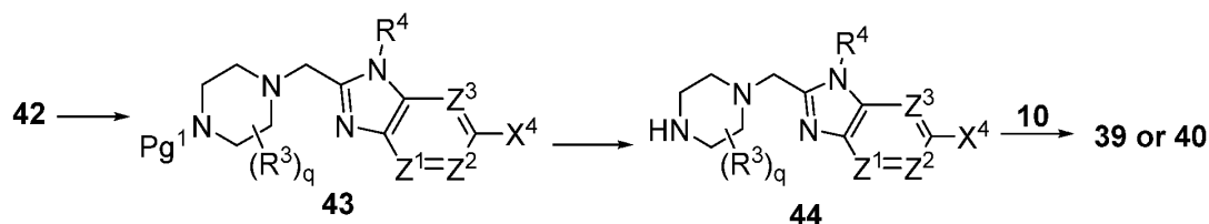
Scheme 11
