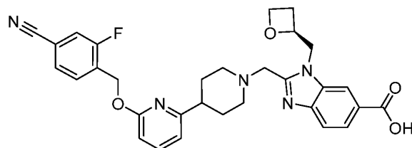
Example 4A-01
