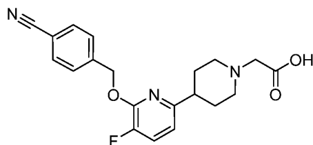
Intermediate 7
