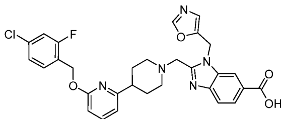
Example 10A-01
