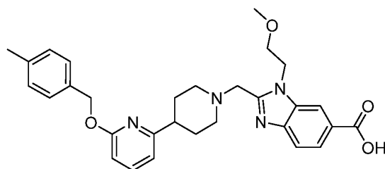
Example 8A-01
