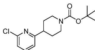
Intermediate 2
