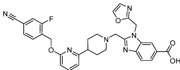
Example 7A-01
