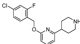
Intermediate 3
