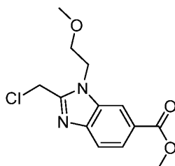
Intermediate 19
