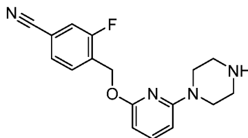
Intermediate 13
