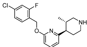
Intermediate 12a
