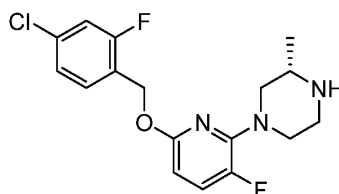
Intermediate 15
