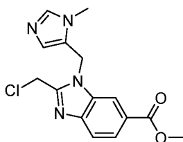
Intermediate 32
