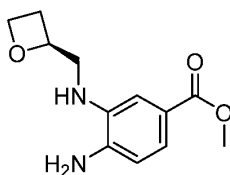
Intermediate 22
