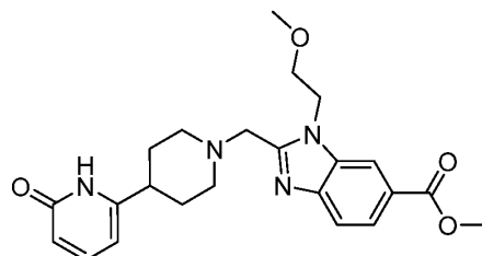
Intermediate 35
