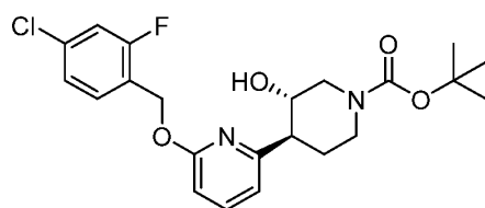
Intermediate 8
