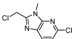
Intermediate 33
