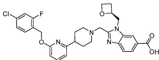
Example 3A-01
