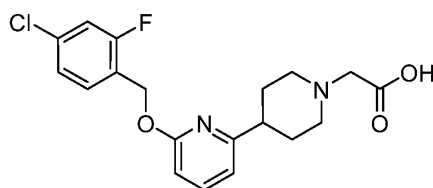
Intermediate 5
