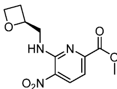
Intermediate 25
