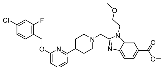
Intermediate 34
