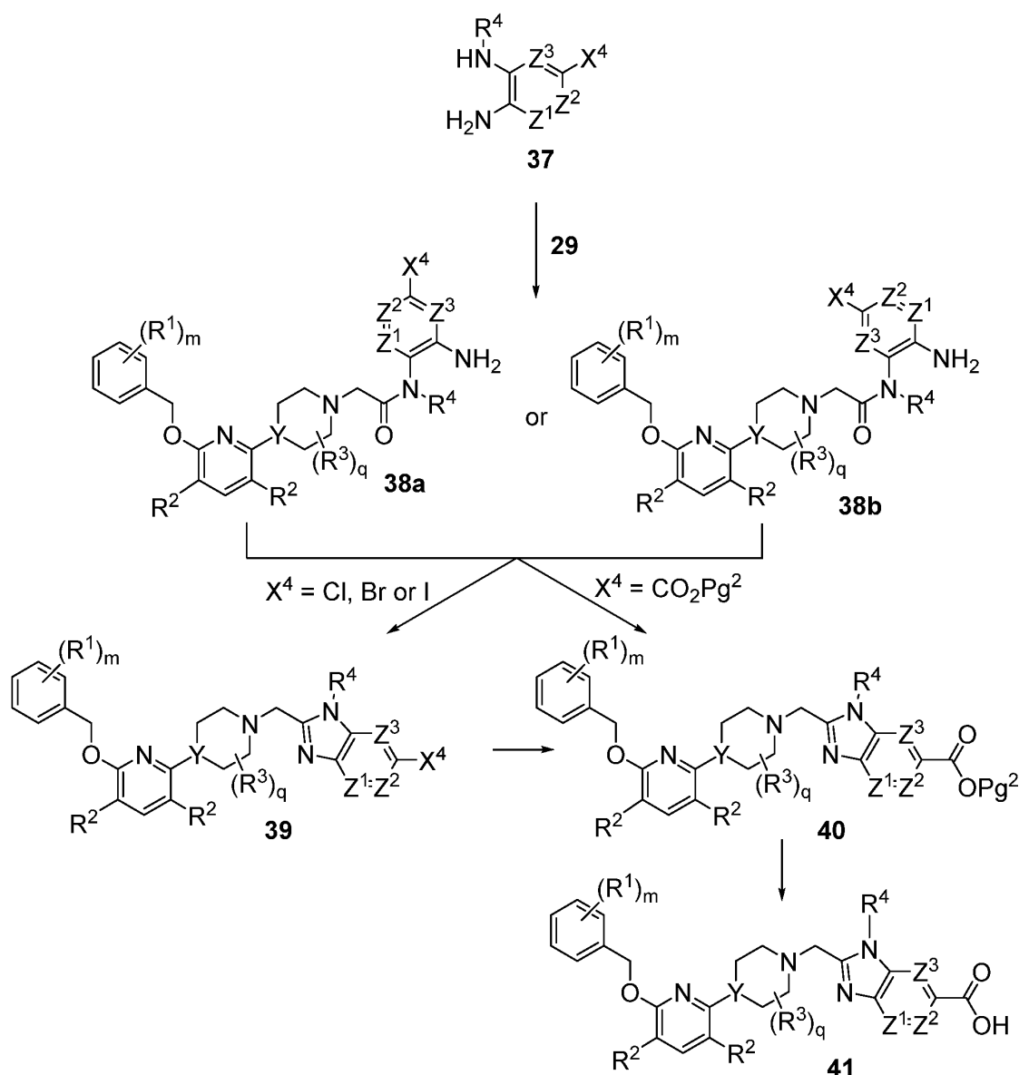
Scheme 9
