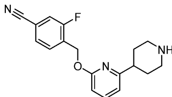
Intermediate 4
