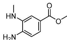
Intermediate 16
