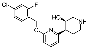
Intermediate 11
