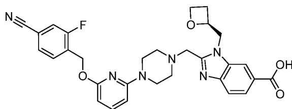
Example 5A-01
