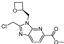
Intermediate 27
