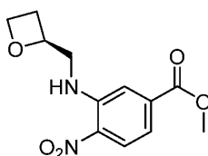
Intermediate 21
