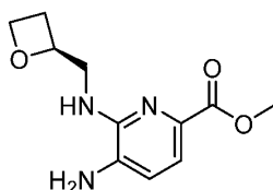
Intermediate 26
