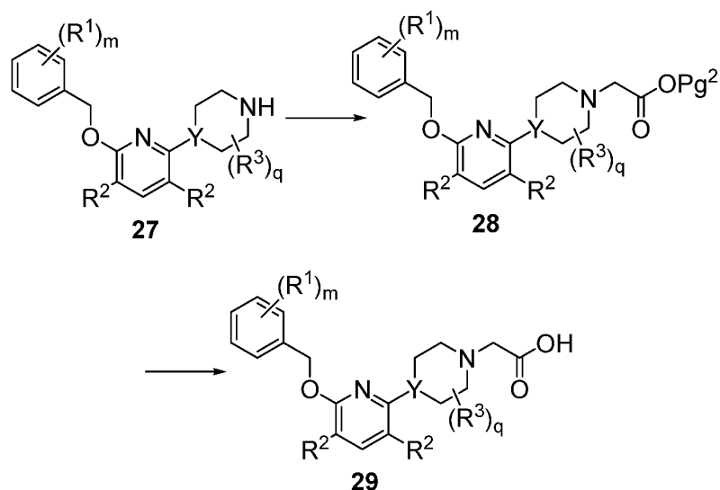
Scheme 7
