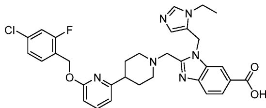
Example 10A-02
