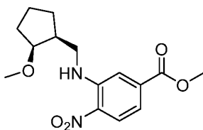
Intermediate 28
