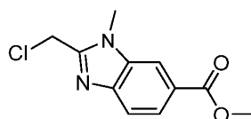
Intermediate 17
