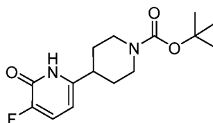
Intermediate 6
