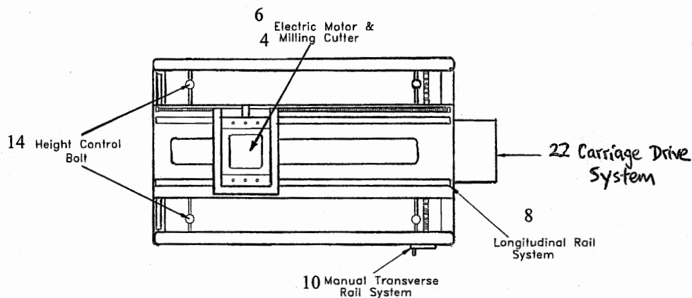
FIGURE 1. IMPROVED PORTABLE MILLER (PLAN VIEW)
