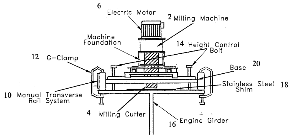
FIGURE 3. IMPROVED PORTABLE MILLER (SIDE VIEW)
