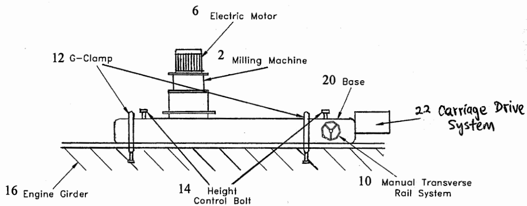
FIGURE 2. IMPROVED PORTABLE MILLER (PROFILE VIEW)
