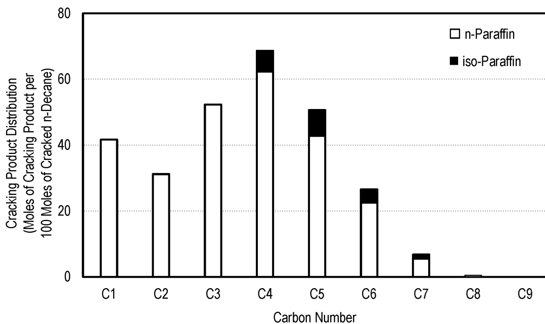
FIG. 6 Cracking Product Distribution at 59.9 mol % of Cracking Yield
