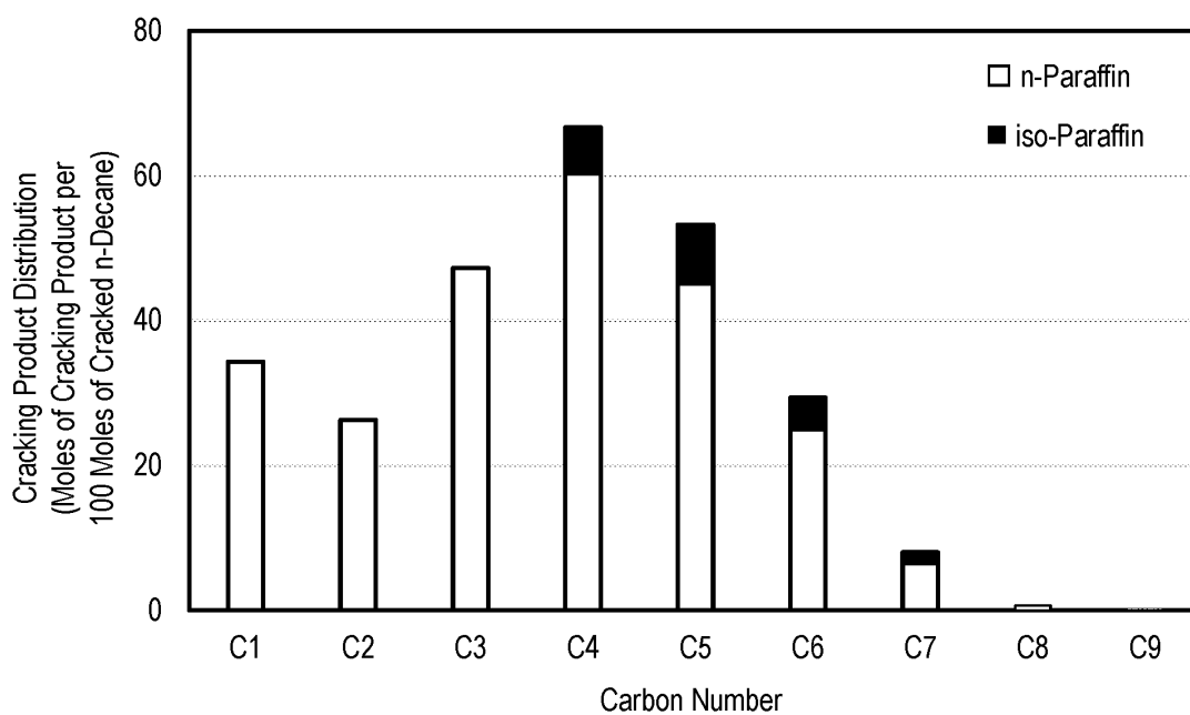
FIG. 4 Cracking Product Distribution at 31.0 mol % of Cracking Yield
