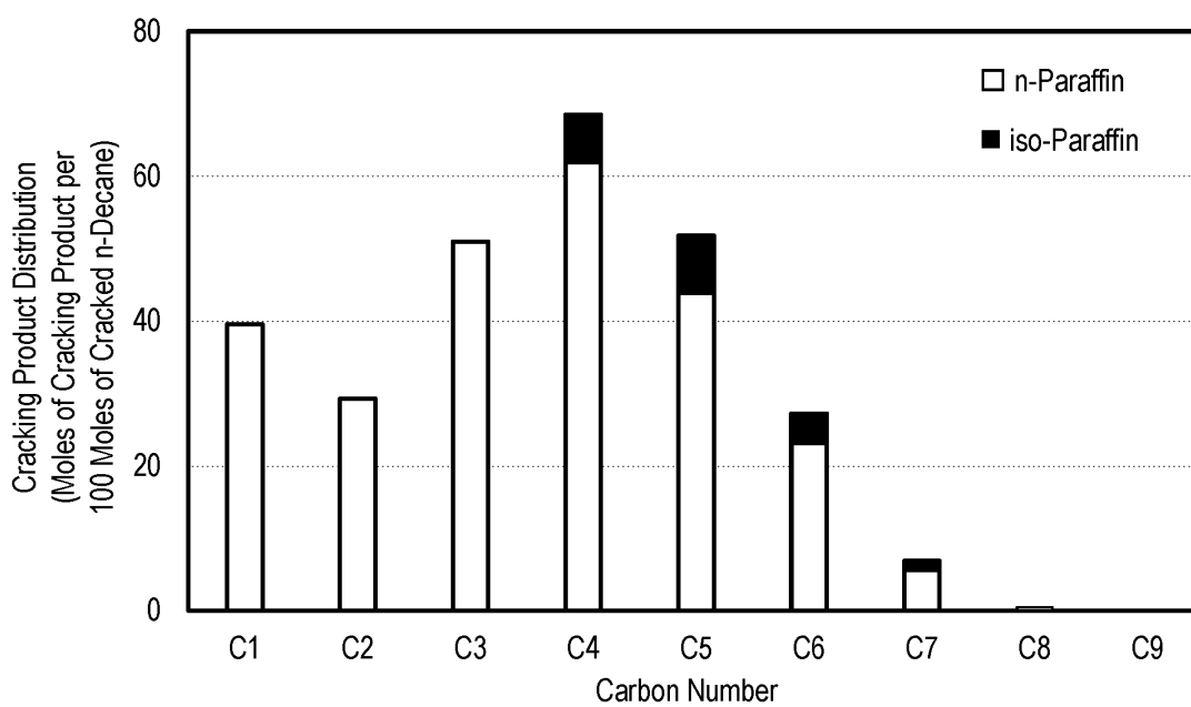
FIG. 5 Cracking Product Distribution at 45.7 mol % of Cracking Yield
