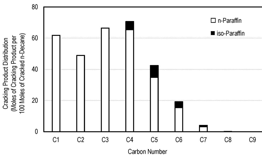
FIG. 7 Cracking Product Distribution at 89.1 mol % of Cracking Yield
