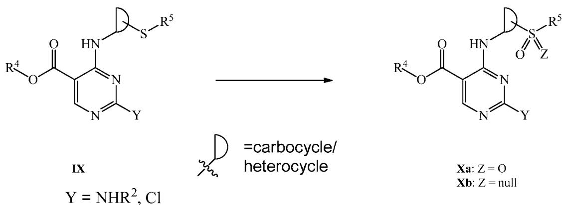
Scheme 5. Oxidation of pendant sulfides IX to Sulfones and Sulfoxides
