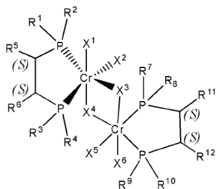
(S), (S)-Chiraphos-bis Chromium complex
