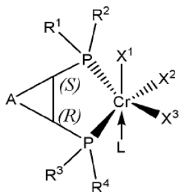
1,2-(R), (S)-cis-Cyclophos-mono Chromium complex
