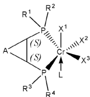
1,2-(S), (S)-trans-Cyclophos-mono Chromium complex
