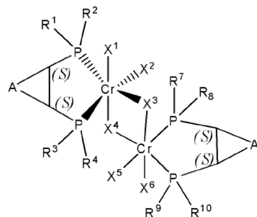
5 1,2-(S), (S)-trans-Cyclophos-bi Chromium complex
