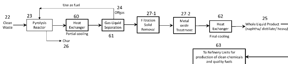
Figure 2 Filtration and Metal Oxide Treatment at Pyrolysis Production Facility for Waste Plastics Pyrolysis Oil for Refinery Unit Co-Feeding
