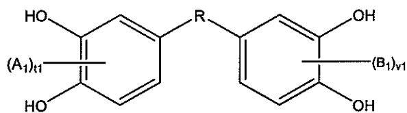
2,4-bis(3,4-dihydroxybenzyl)-8-methyl-8-aza-bicyclo[3.2.1]octan-3-one
