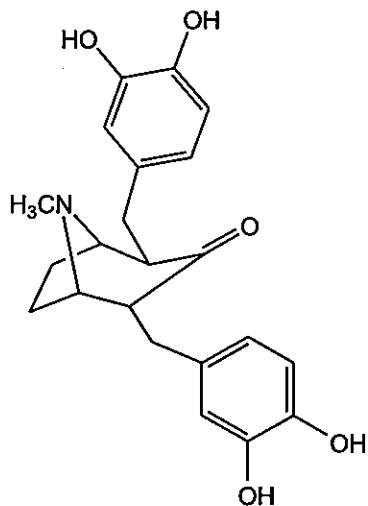
2,4-bis(3,4-dihydroxybenzyl)-8-methyl-8-aza-bicyclo[3.2.1]octan-3-one
