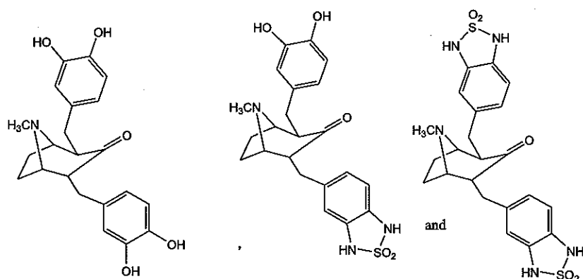
2,4-bis(3,4-dihydroxybenzyl)-8-methyl-8-aza-bicyclo[3.2.1]octan-3-one
