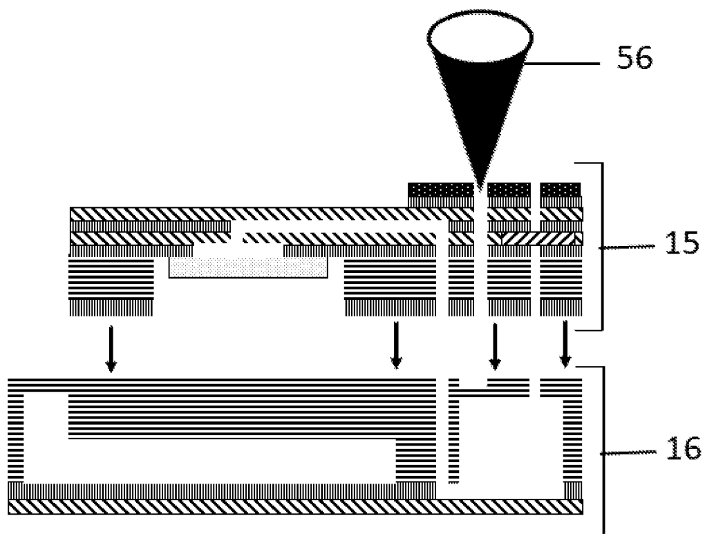
Potential Layer Stackup Illustration
