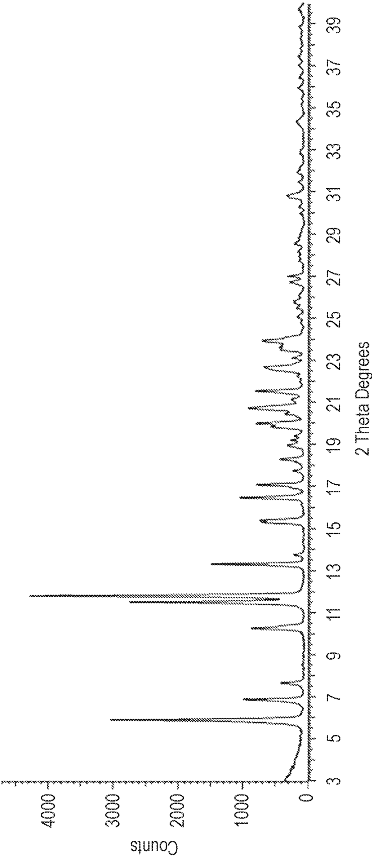
FIG. 2 PXRD pattern of crystalline sodium salt of Example 5
