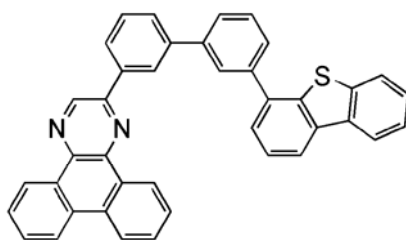
2mDBTBPDBq-II
