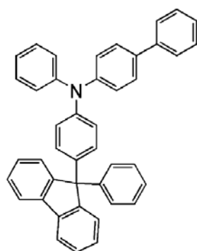
BPAFLP
