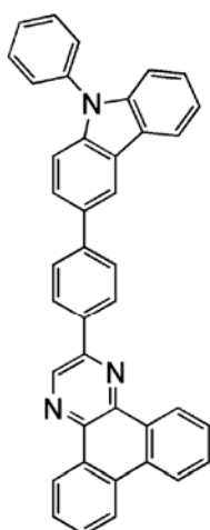
PCPDBq
