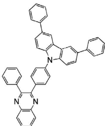
Cz1PQ-III
