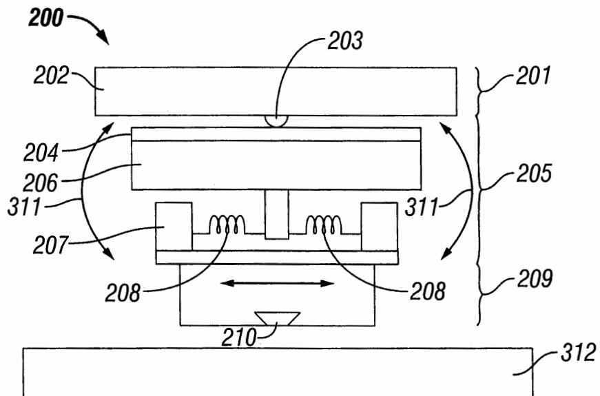
FIG. 3 (Prior Art)
