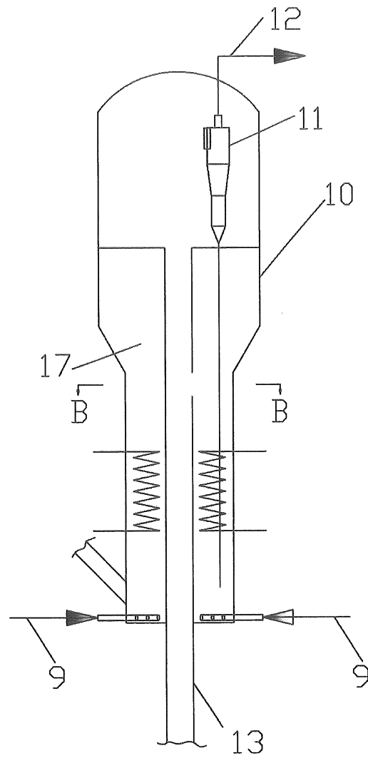
B-B section
