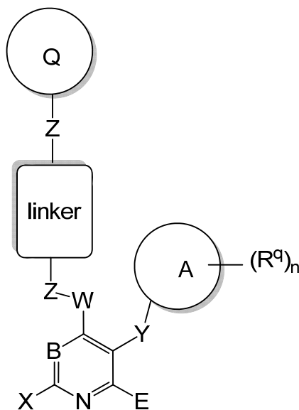
Formula (II),
