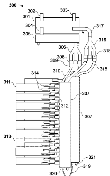
FIG. 3 (Schematic of the two-phase cooling system.)
