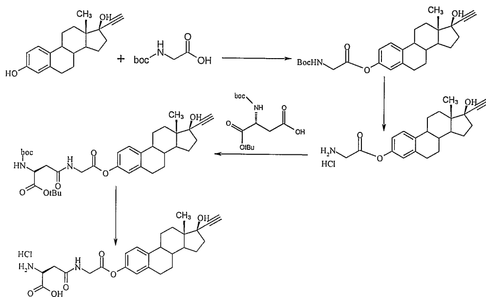
Reaction Sequence 10
