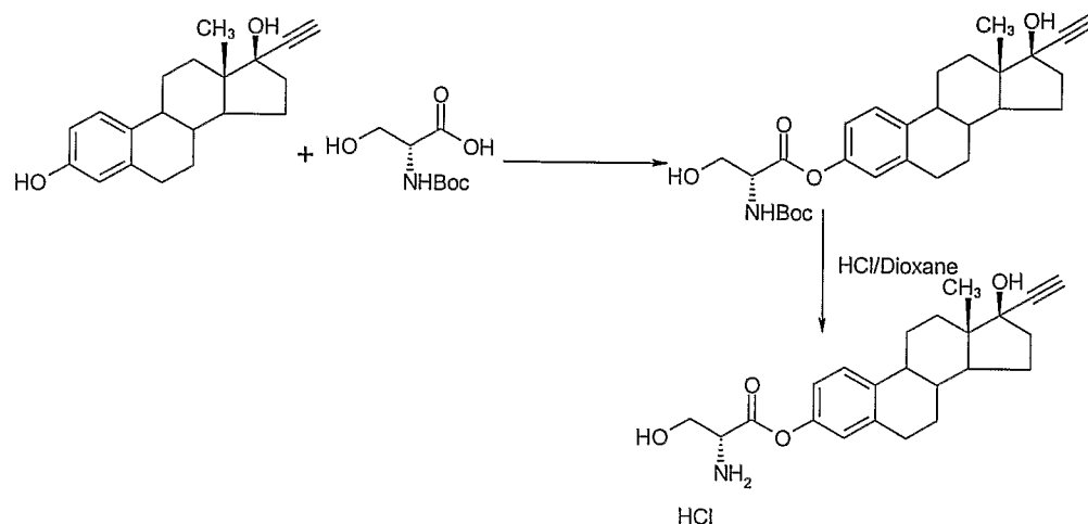
Reaction Sequence 7
