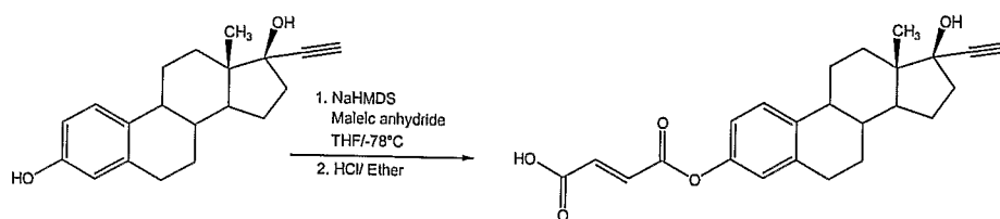
Reaction Sequence 1
