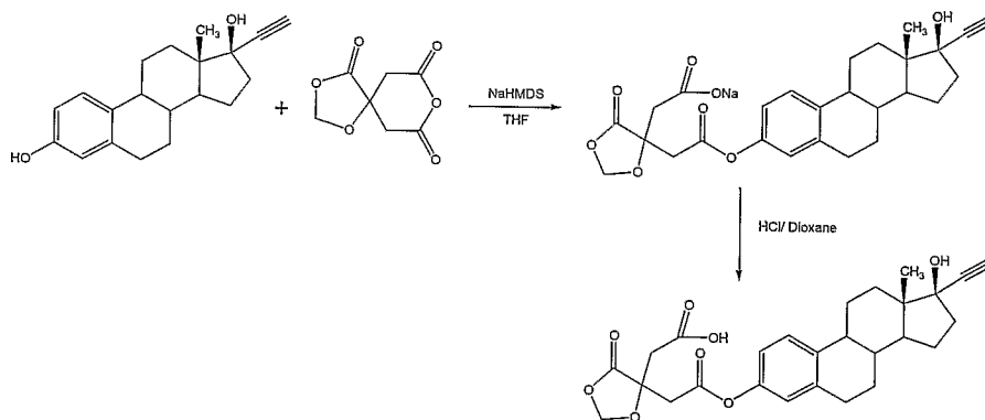
Reaction Sequence 2
