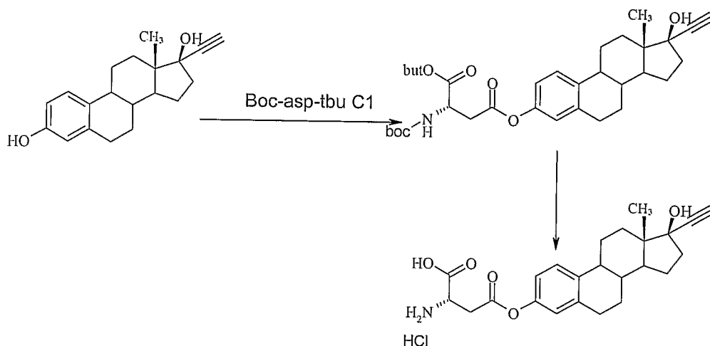
Reaction Sequence 12
