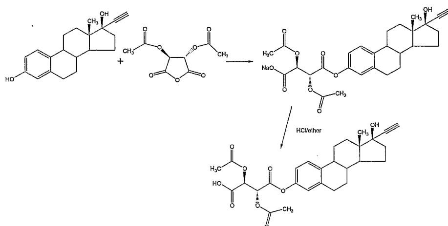
Reaction Sequence 9
