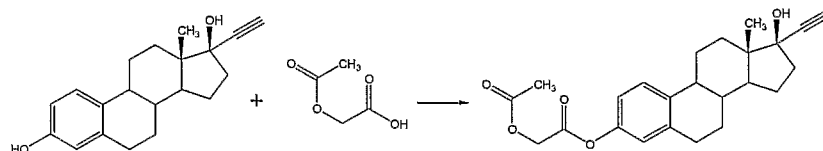
Reaction Sequence 5
