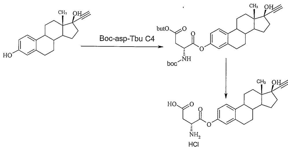
Reaction Sequence 11
