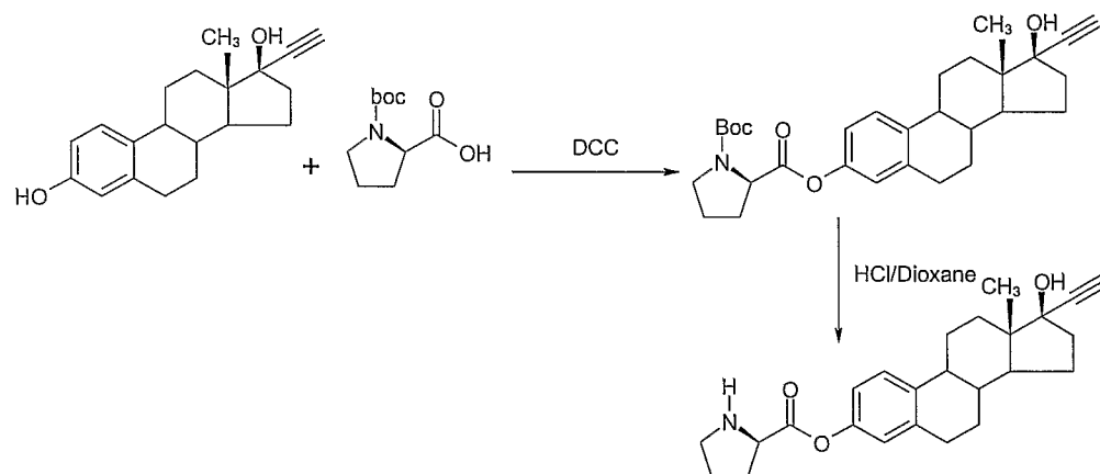
Reaction Sequence 6
