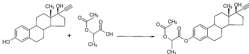
Reaction Sequence 8
