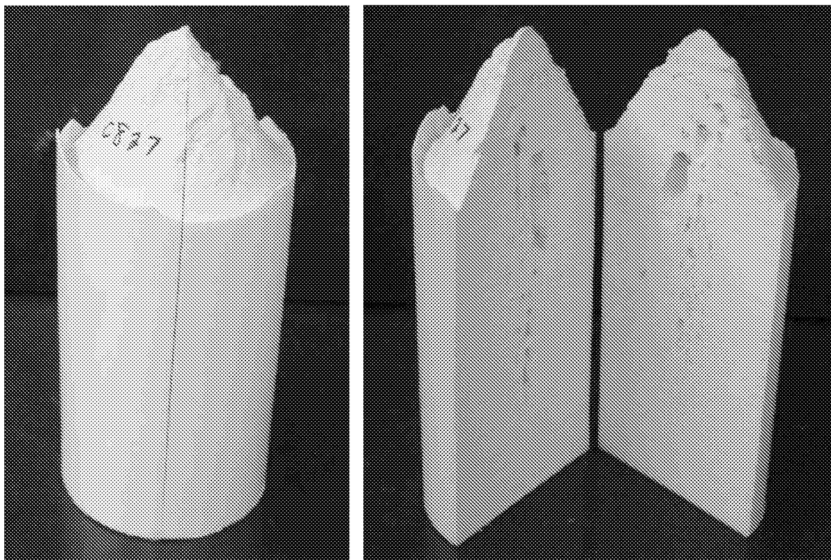
FIG. 3 Photographs of an article made from a cyclic olefin resin composition catalyzed with a single metal carbene olefin metathesis catalyst, according to Example 61, showing the presence of defects.
