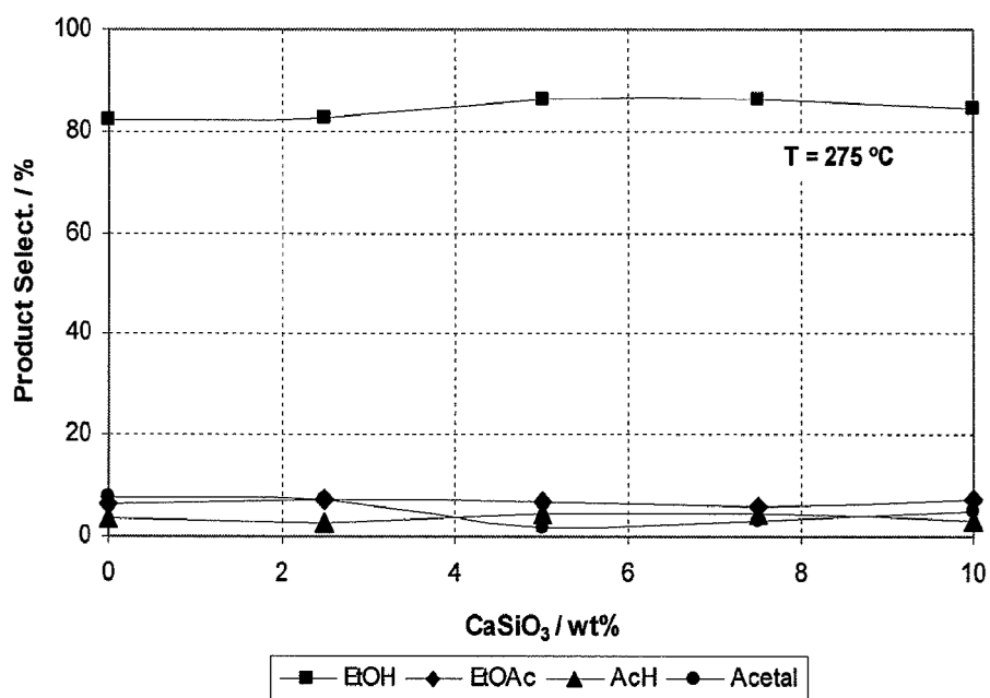
FIG. 6D - Selectivity @ 275
