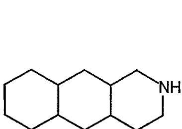
Perhydrobenzo(g)isoquinoline
