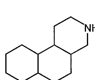
Perhydrobenzo(f)isoquinoline
