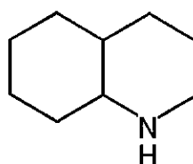
Perhydroquinoline
