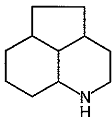
Perhydroacequinoline
