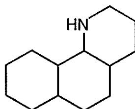
Perhydrobenzo(h)quinoline
