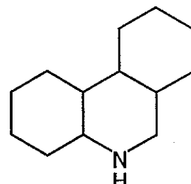
Perhydrophenanthridine
