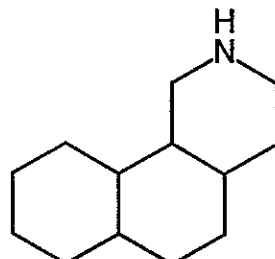
Perhydrobenzo(h)isoquinoline
