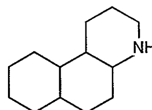
Perhydrobenzo(f)quinoline
