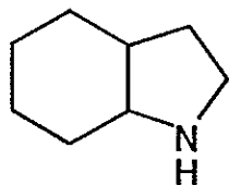
Perhydroindole
