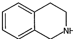
1,2,3,4-tetrahydroisoquinoline
