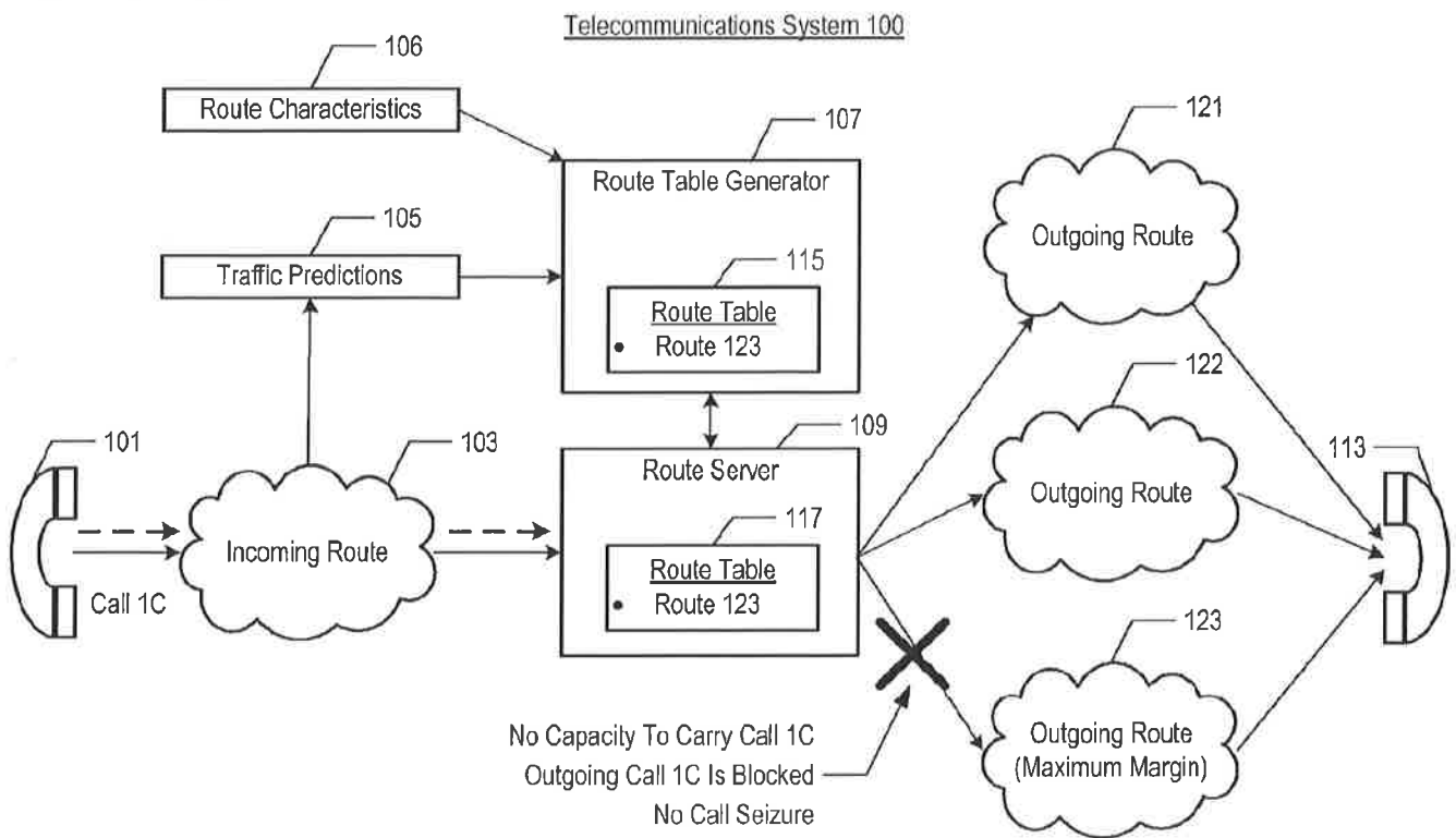
Figure 1C (Prior Art)
