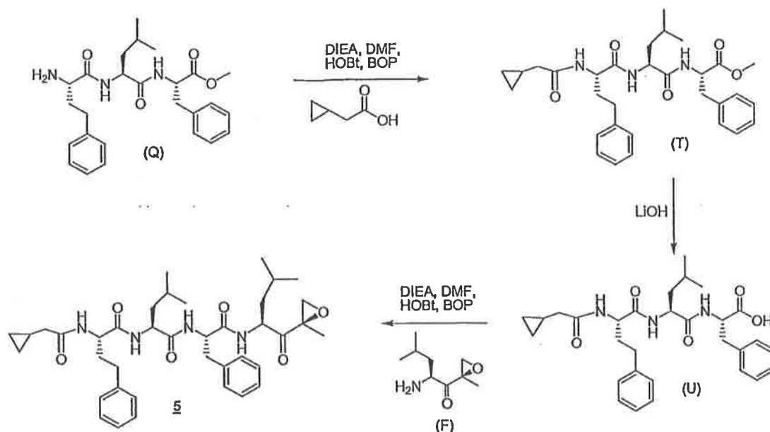
Scheme 5: Synthesis of Example 5
