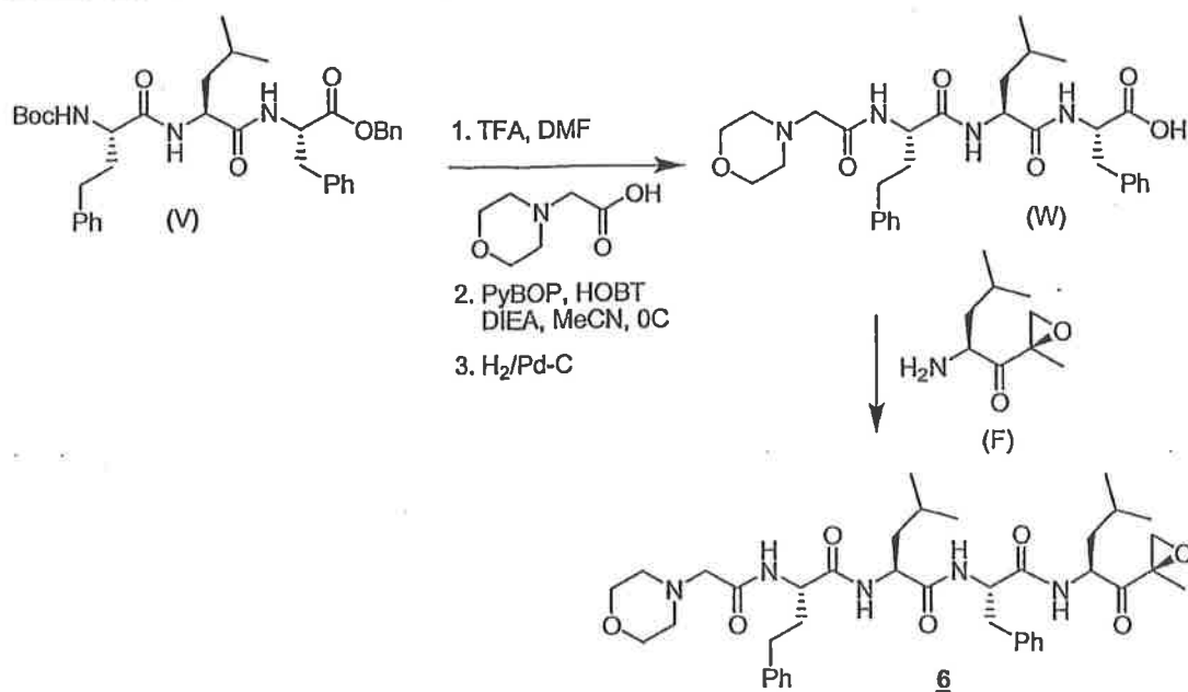
Scheme 6. Synthesis of Example 6
