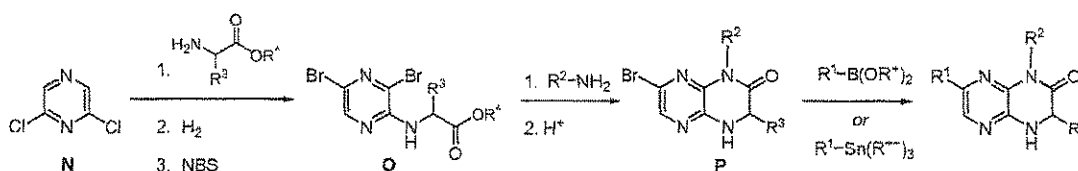
Scheme 8
