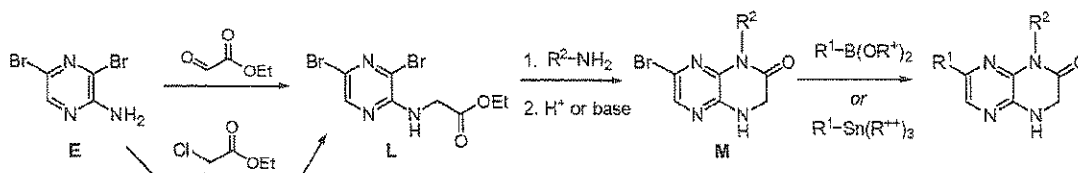
Scheme 7
