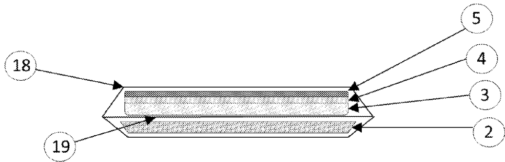
Figure 6 – Heating Process in a Microwave
