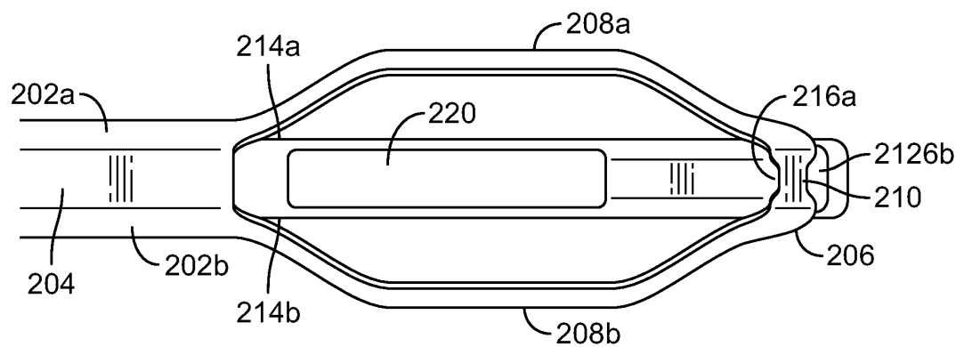
FIG. 9C SUBSTITUTE SHEET (RULE 26)
