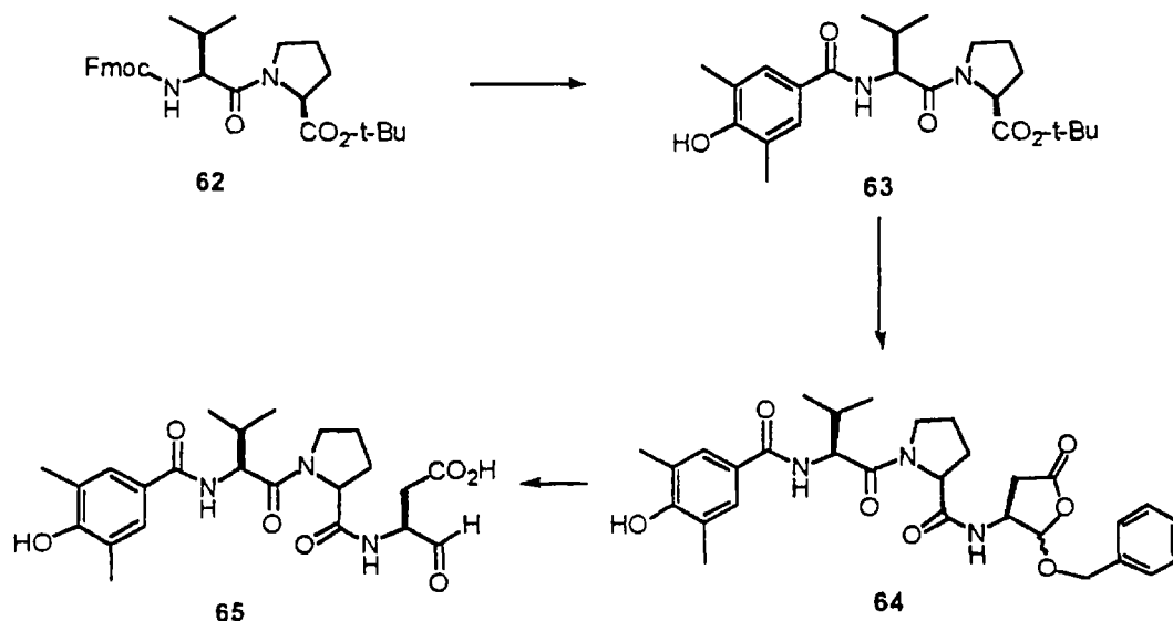
Scheme XIII
