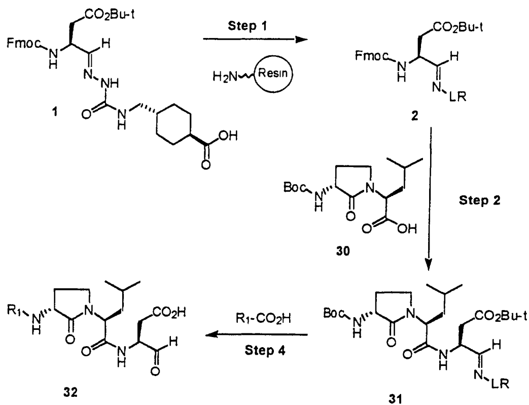
Scheme VII
