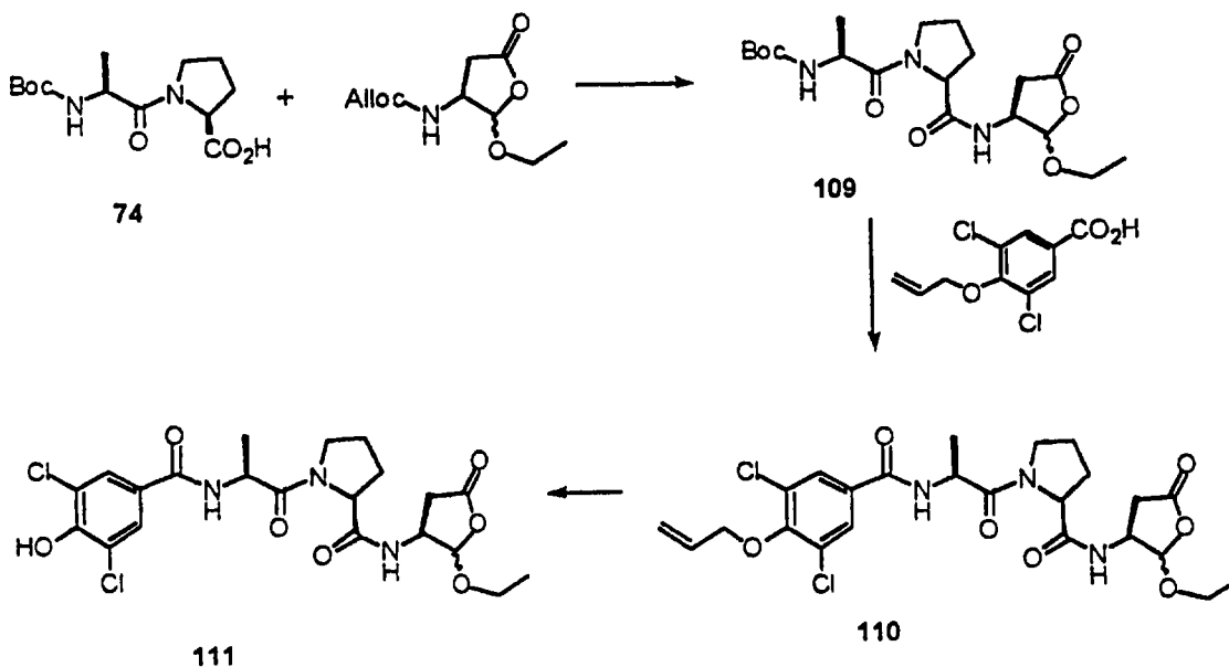
Scheme XX
