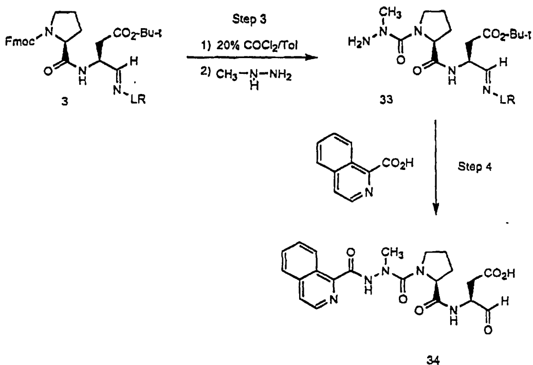
Scheme VIII
