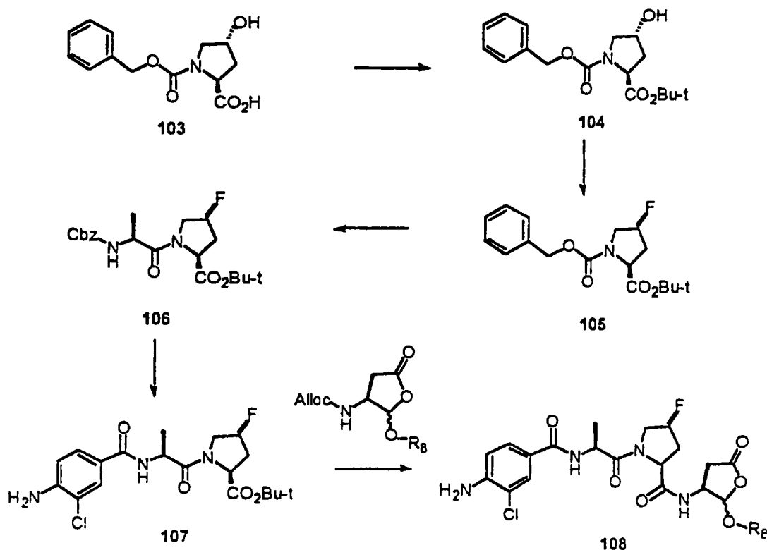
Scheme XIX
