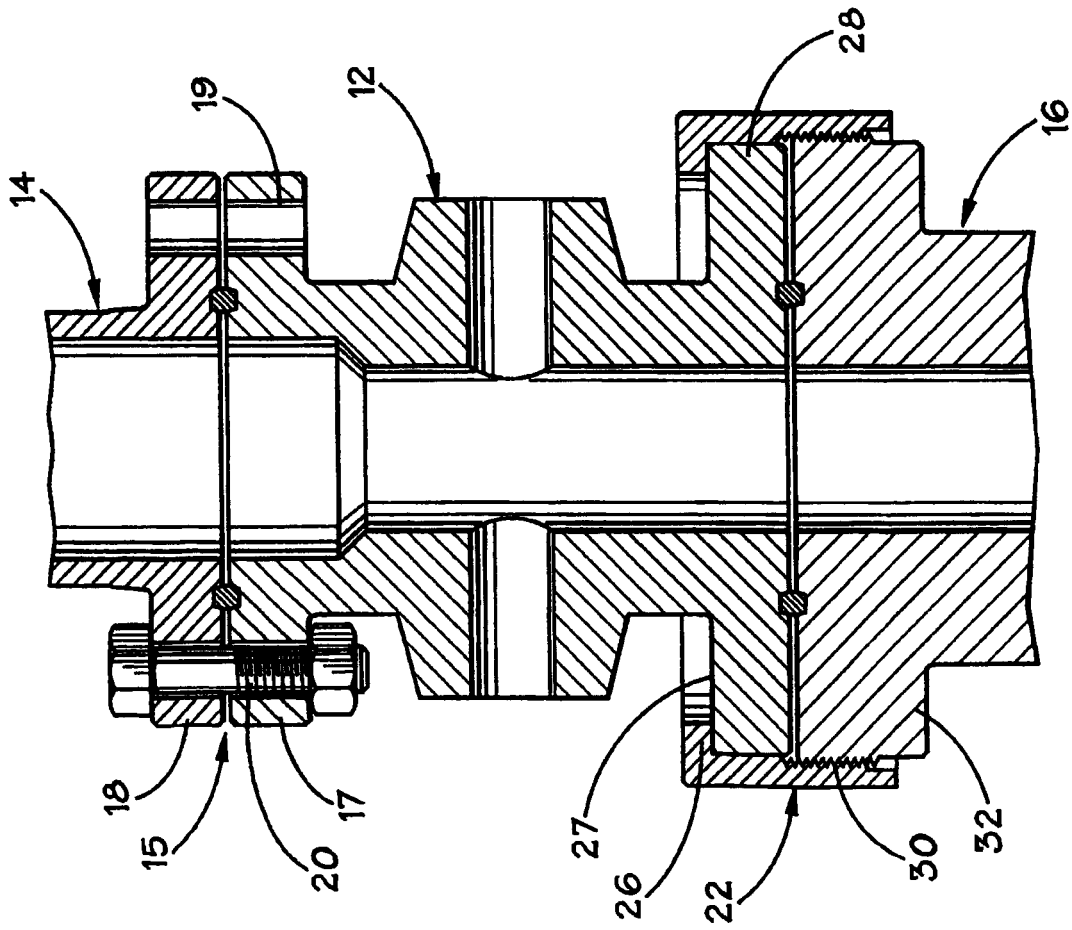
FIG. 1 (PRIOR ART)
