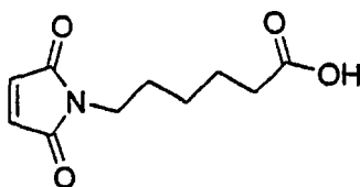
6-maleimidocaproic acid
