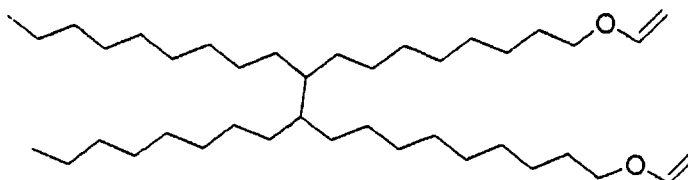
"Dimer Divinyl Ether" (and cyclic isomers)
