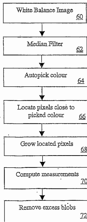
Figure 5 Mitosis Feature Detection
