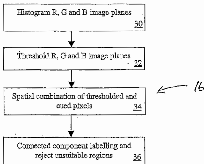
Figure 2 Mitosis feature cueing
