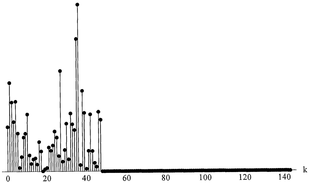
ZERO-PADDED POWER SPECTRUM OF ORIGINAL CHANNEL ESTIMATE
