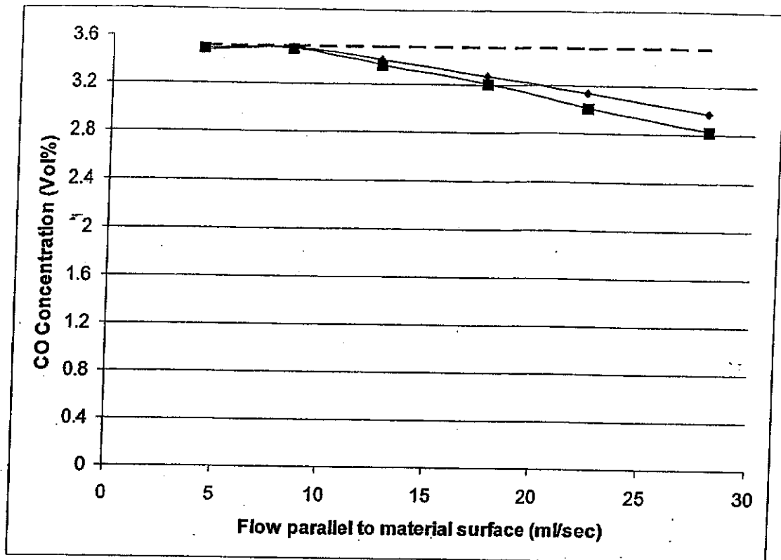
Graph 1: Legend: - - - Maximum concentration in equilibrium; ■ polypropylene membrane; ◆ polyethylene membrane.
