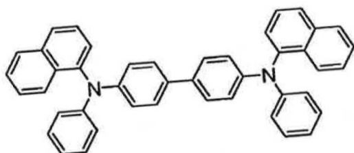
NPB
