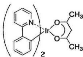
\text{Ir}(\text{ppr})_2\text{acac}
