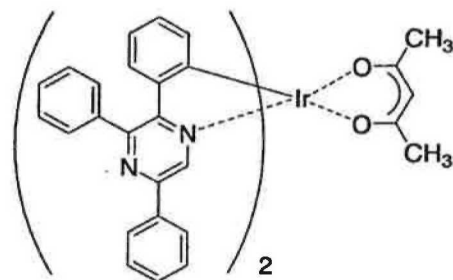
\text{Ir}(\text{tppr})_2\text{acac}
