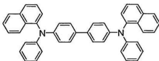
NPB
