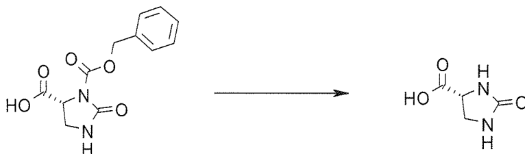
(2) (R)-2-Oxoimidazolidine-4-carboxylic acid
