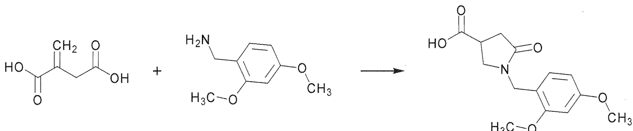
(1) 1-(2,4-Dimethoxybenzyl)-5-oxopyrrolidine-3-carboxylic acid
