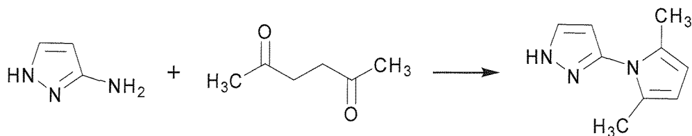
(1) 3-(2,5-Dimethylpyrrol-1-yl)-1H-pyrazole
