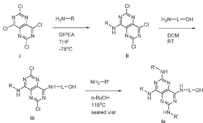
Scheme 4
