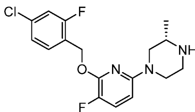
Intermediate 14
