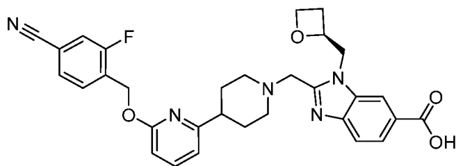
Example 4A-01
