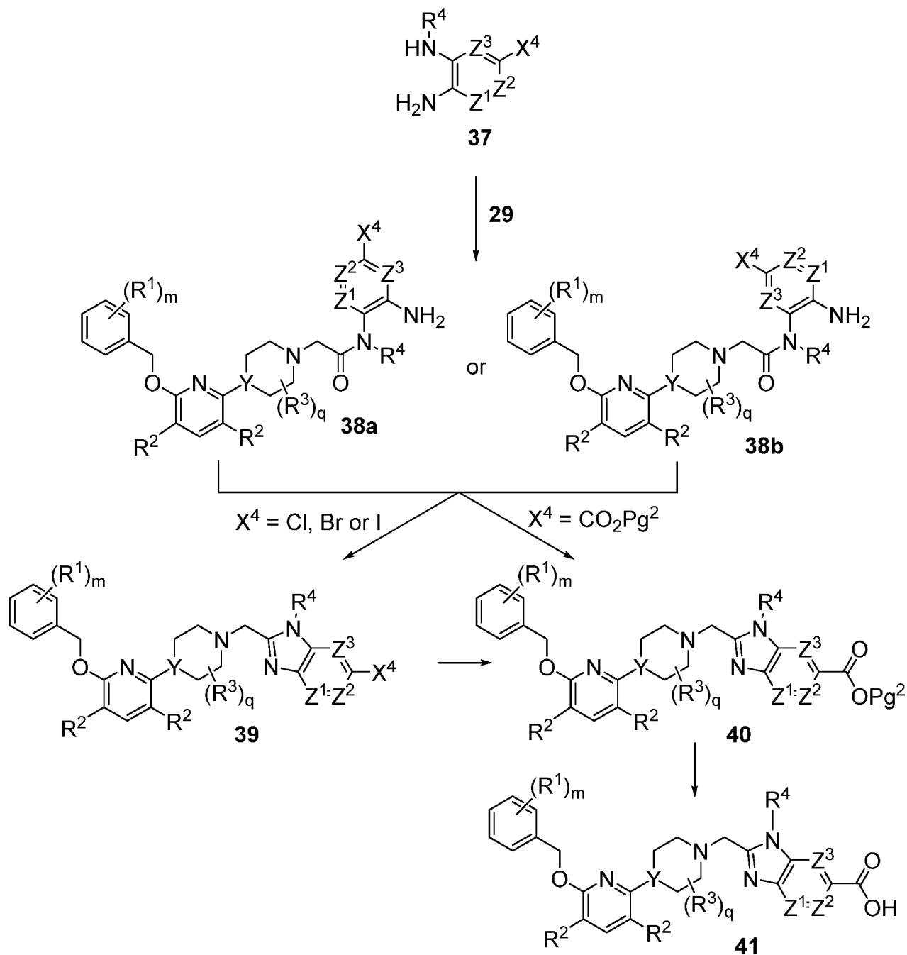
Scheme 9
