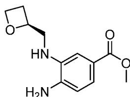
Intermediate 22
