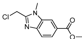
Intermediate 17
