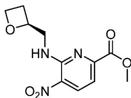
Intermediate 25
