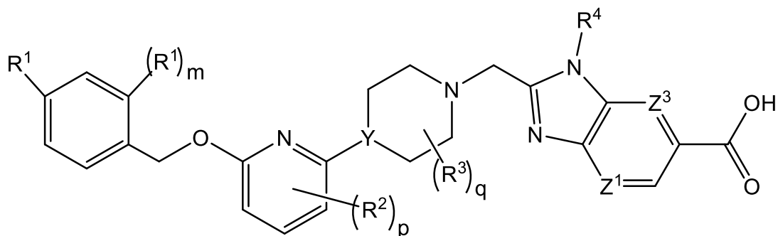
II
