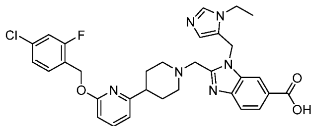
Example 10A-02
