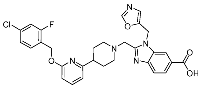
Example 10A-01
