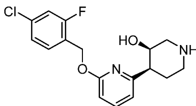
Intermediate 11
