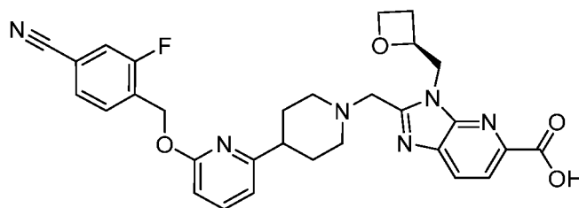
Example 6A-01
