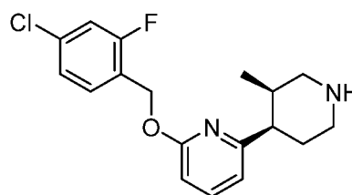
Intermediate 12a
