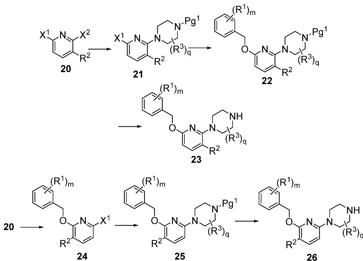
Scheme 6
