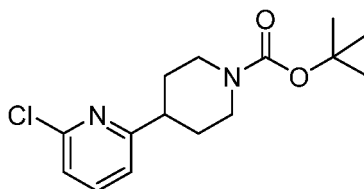
Intermediate 2
