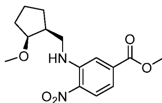
Intermediate 28
