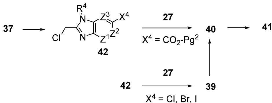
Scheme 10
