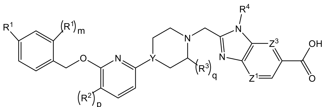
III
