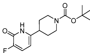
Intermediate 6
