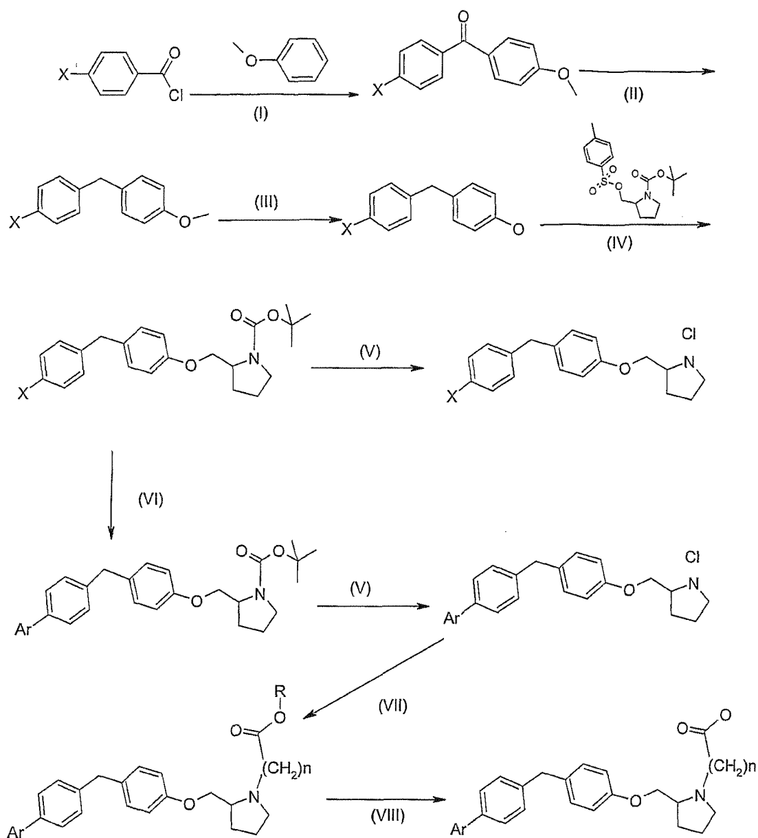
Scheme X: (I) \text{AlCl}_3 , nitrobenzene, (II) \text{Et}_3\text{SiH} , TFA, (III) \text{BBr}_3 , \text{CH}_2\text{Cl}_2 , (IV) \text{NaH} , DMF, (V) \text{HCl} , dioxane, (VI) \text{ArB} \text{Pd}(\text{OAc})_2/\text{PPh}_3/\text{CsCO}_3 , DME/EtOH/ \text{H}_2\text{O} , (VII) \text{Br}(\text{CH}_2)_n\text{CO}_2\text{R} , base, (VIII) \text{NaOH} or \text{HCl} .
