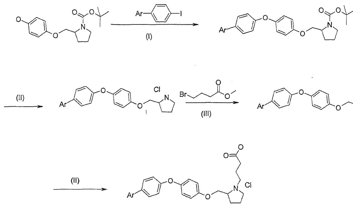
Scheme XV: (I) \text{Cs}_2\text{CO}_3/(\text{CH}_3)_2\text{NCH}_2\text{CO}_2\text{H} , \text{CuI}/\text{dioxane}/98\text{ }^\circ\text{C} , (II) \text{HCl} , dioxane, (III) \text{K}_2\text{CO}_3 , DMF
