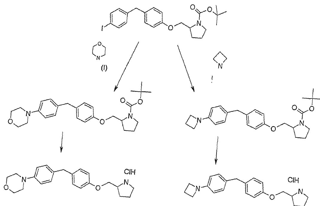
Scheme XI: (I) \text{Pd}_2(\text{dba})_3/\text{t-Bu}_3\text{P} , \text{NaOtBu} /toluene, (II) \text{HCl} , dioxane
