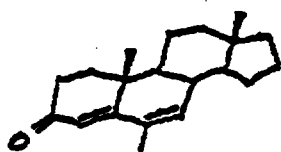
6-METHYLANDROSTA-4,6-DIEN-3-ONE
