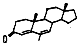
6-METHYLANDROSTA-4,6-DIEN-3-ONE
