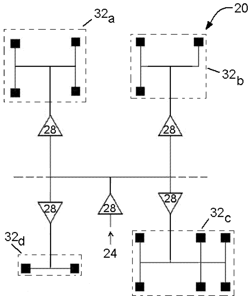
Fig. 1 (Prior Art)
