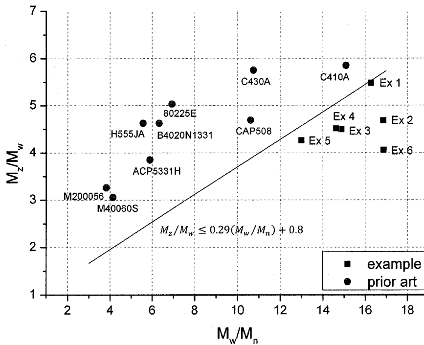
Figure 4 M_z/M_w vs. M_w/M_n
