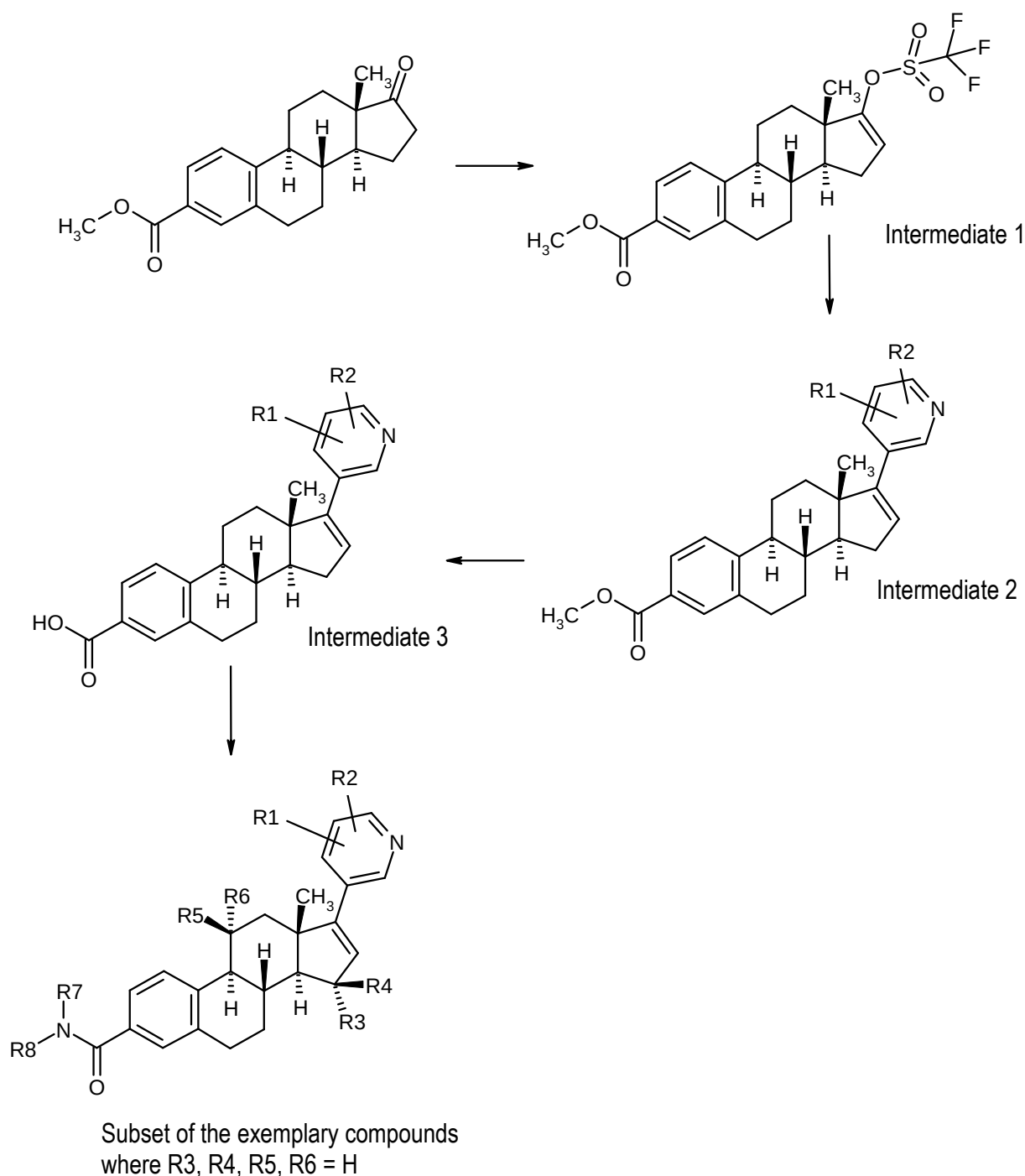
Synthesis scheme 1
