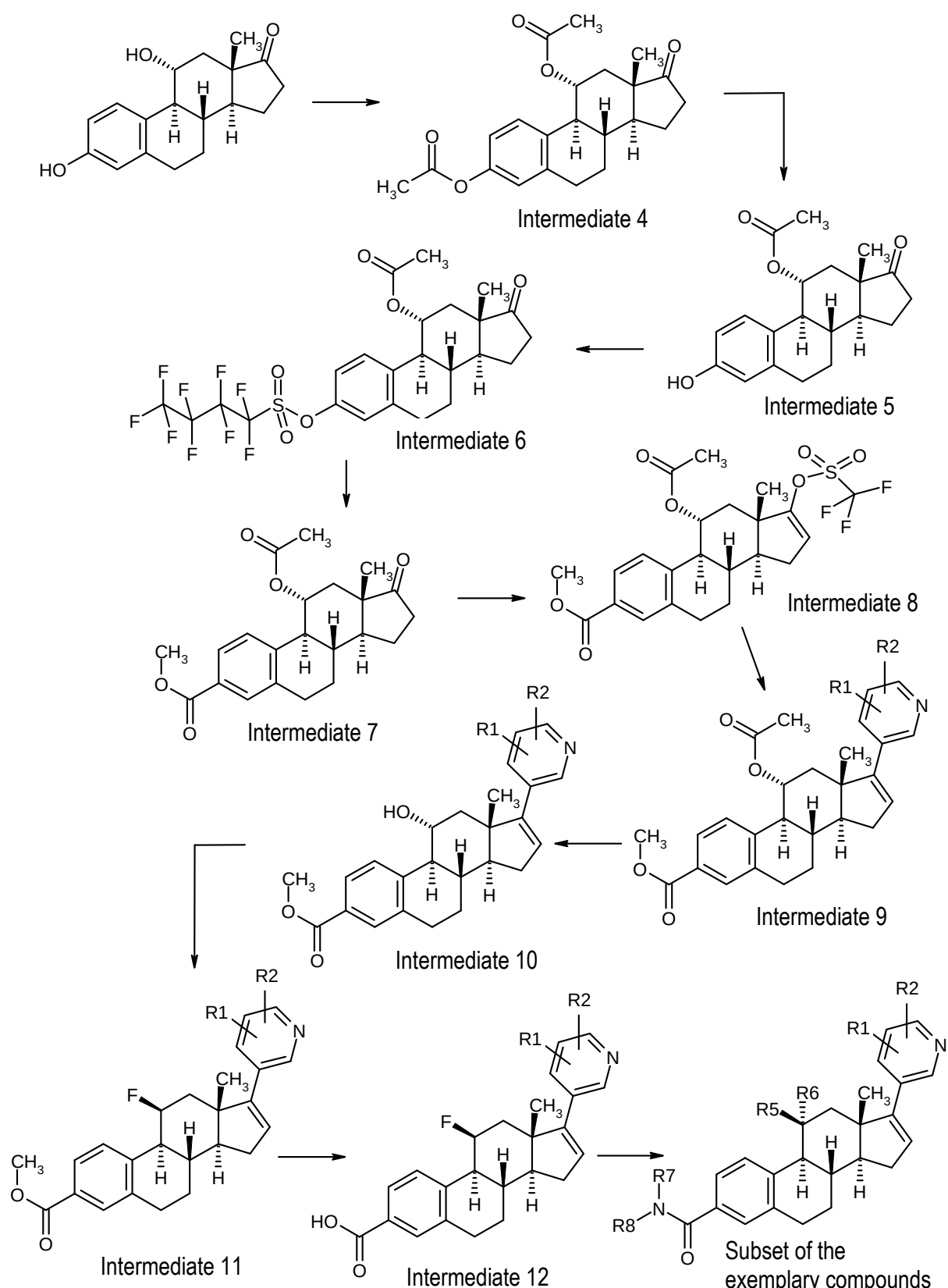
Synthesis scheme 2
