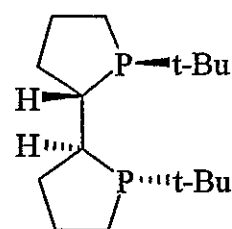
( R,R,S,S )-"TangPhos"
